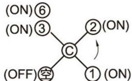
SCHEMATIC (NON-SHORTING)
